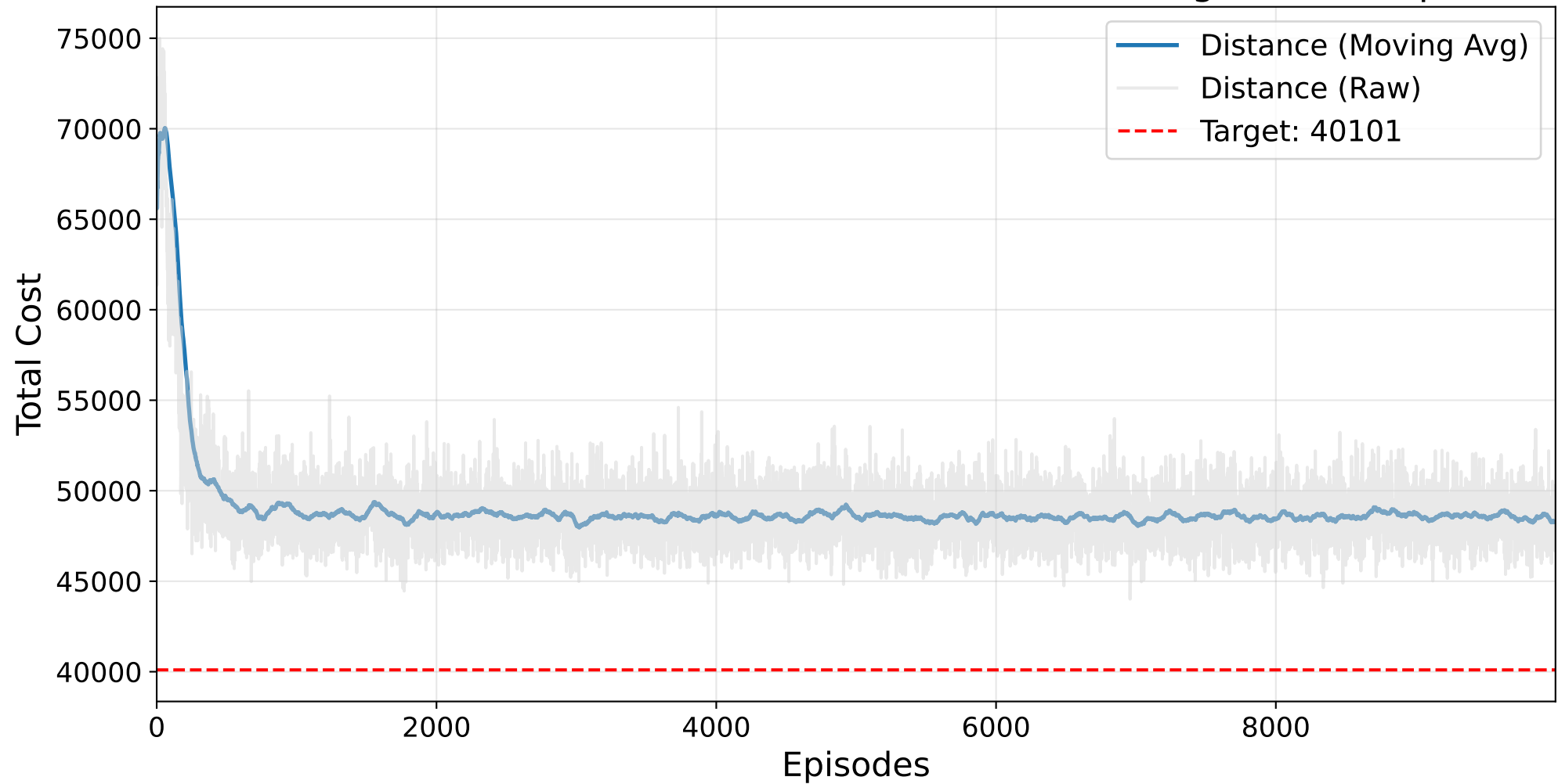
Final HYPERBAND GP Masked AutoRL-SOP Training - ft70.2.sop
